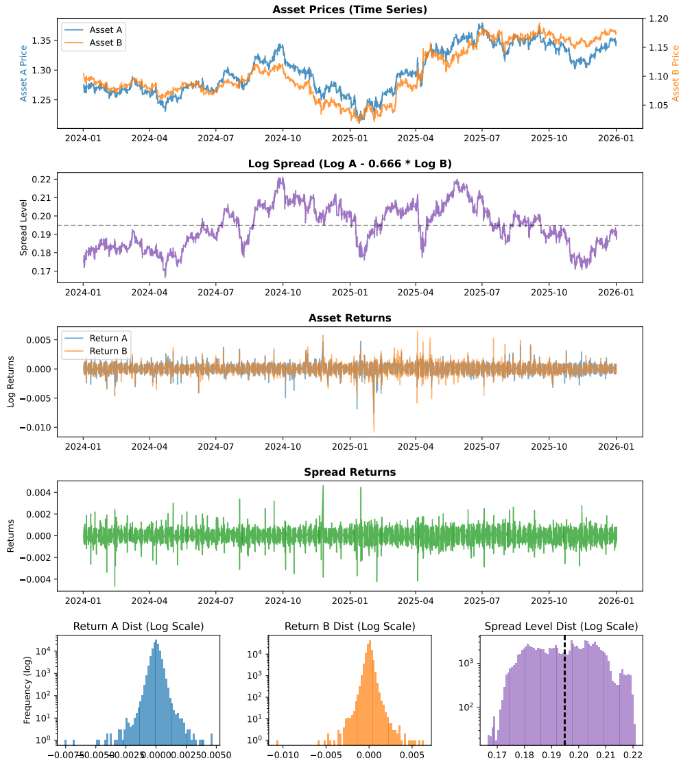
Figure 6: Spread diagnostics for GBPUSD/EURUSD. The figure shows the two asset price series, estimated log spread, asset returns, spread returns, and distributional diagnostics, providing a visual basis for assessing the stability and tradability of the constructed spread.
