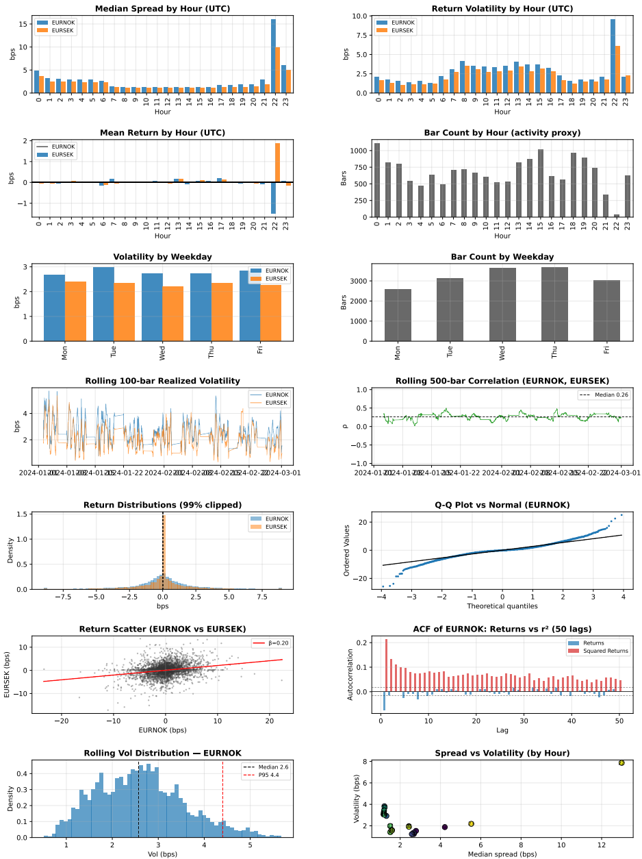
Figure 2: Exploratory data analysis for EURNOK/EURSEK. The figure summarizes intraday spreads, volatility, mean returns, bar counts, weekday effects, rolling realized volatility, rolling correlation, distributional features, normality diagnostics, cross-pair return scatter, autocorrelation, rolling volatility, and the spread-volatility relationship.
