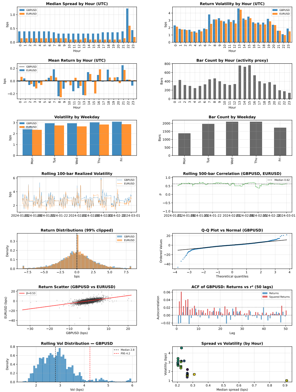
Figure 3: Exploratory data analysis for GBPUSD/EURUSD. The figure summarizes intraday liquidity and volatility patterns, hourly and weekday activity, rolling realized volatility, rolling correlation, return distributions, normality diagnostics, cross-pair return dependence, autocorrelation, and the relationship between spread and volatility.
