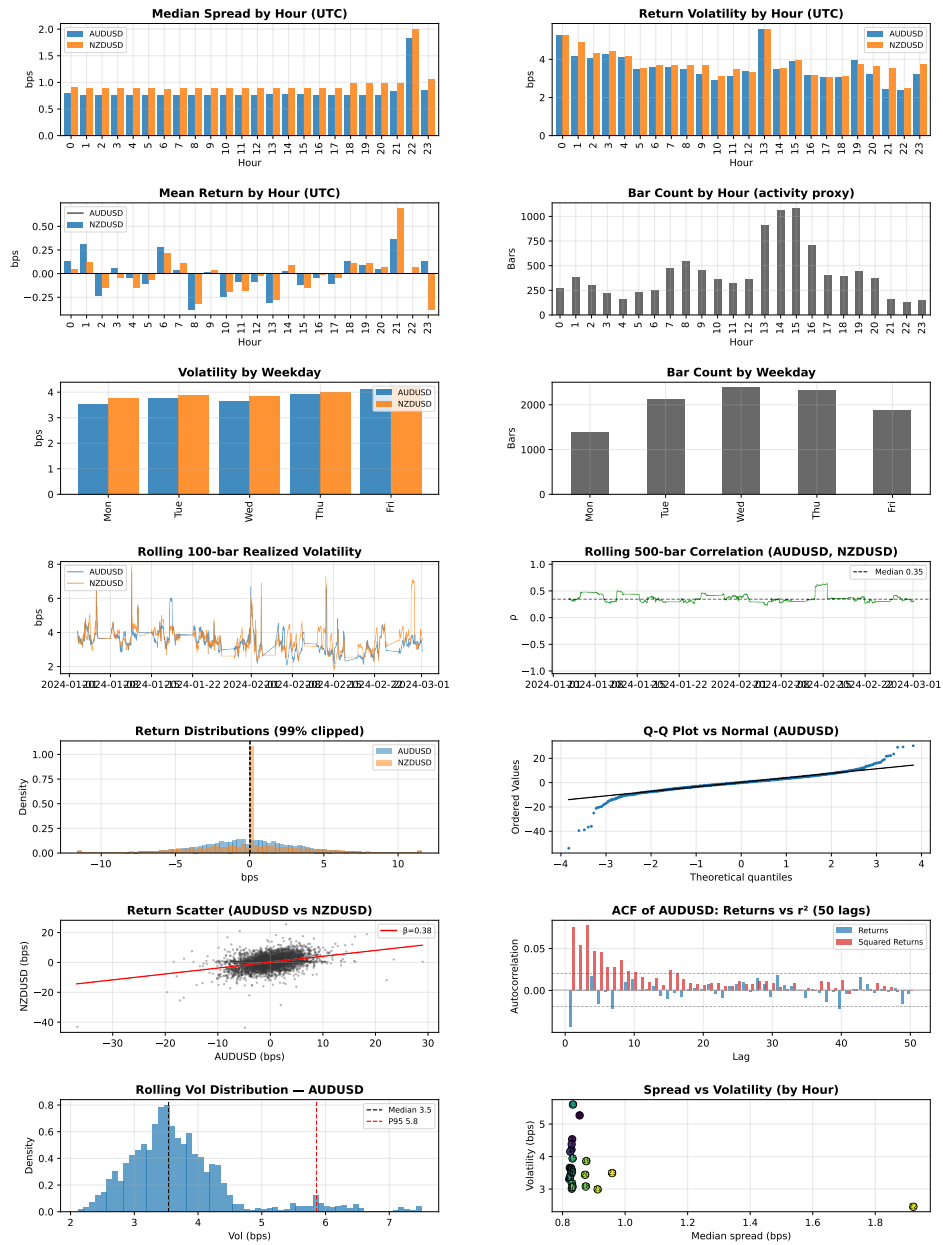
Figure 1: Exploratory data analysis for AUDUSD/NZDUSD. The figure summarizes intraday spreads, return volatility, mean returns, activity patterns, weekday effects, rolling realized volatility, rolling correlation, return distributions, normality diagnostics, cross-pair return scatter, autocorrelation, rolling volatility distribution, and the relationship between spread and volatility.
